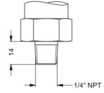
1/4" NPT
